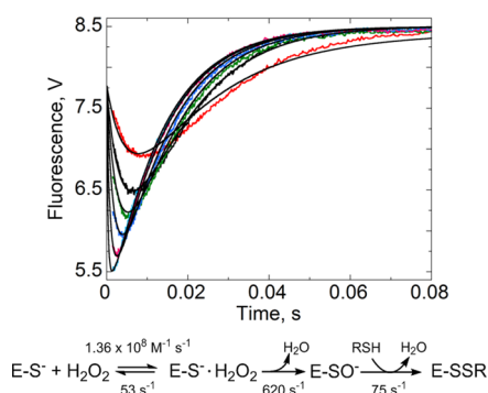
Figure 4. Kinetic model for fitting AhpC fluorescence changes after addition of \text{H}_2\text{O}_2 . KinTek Global Kinetic Explorer was used to test kinetic models and conduct fits to the data as described in the text. The best fits to the global model are the black lines shown with the experimental data (gathered as in Figure 3a) at various \text{H}_2\text{O}_2 concentrations, colored red (1 \mu\text{M} ), black (2 \mu\text{M} ), green (3 \mu\text{M} ), blue (5 \mu\text{M} ), magenta (10), and cyan (25 \mu\text{M} ). The kinetic model to which these data fit best and our interpretation of the reaction steps detected are depicted below the plot.
