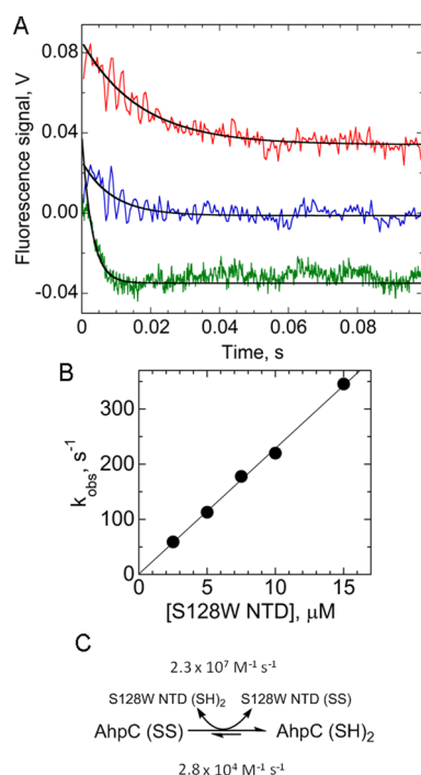
Figure 2. Reduction of AhpC by the redox-sensing mutant of the AhpF N-terminal domain (S128W NTD). (A) To assess rates of reduction of AhpC, oxidized AhpC (1 μM for 2.5–10 μM S128W NTD and 3 μM for >10 μM S128W NTD) was mixed with reduced S128W NTD at 2.5 (red), 5 (blue), and 15 μM (green), monitoring fluorescence changes in both proteins over time ( \lambda_{\text{ex}} = 280 \text{ nm} ; \lambda_{\text{em}} > 320 \text{ nm} ). Red and blue curves have been displaced upward on the y-axis for the sake of clarity; amplitudes of change were somewhat variable in these averaged, noisy spectra, but the data were readily fit to a single-exponential equation. (B) Pseudo-first-order rate constants obtained from the fits in panel A, plotted vs S128W NTD concentration, yield a second-order rate constant of 2.3 \times 10^7 \text{ M}^{-1} \text{ s}^{-1} . (C) Reaction pathway annotated with rate constants.
