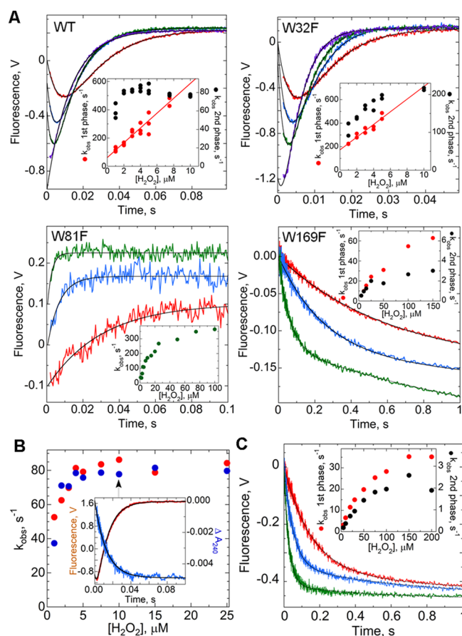
Figure 3. Kinetic profiles of intrinsic Trp fluorescence and absorbance changes of wild-type and mutant AhpC during H 2 O 2 -mediated oxidation. (A) Reduced AhpC (1 μM) in reaction buffer [25 mM potassium phosphate (pH 7) with 1 mM EDTA and 100 mM ammonium sulfate] at 25 °C was mixed in a stopped-flow spectrofluorometer with increasing concentrations of H 2 O 2 , with representative traces colored red, blue, green, and purple (1, 3, 5, and 20 μM for the wild type, 1, 3, 5, and 15 μM for W32F, 2, 10, and 100 μM for W81F, and 2, 4, and 25 μM for W169F). All concentrations are after mixing. All data (except for W81F) fit to a double exponential (black lines) yielded rate constants for the fast (red) and slow (black) phases, plotted vs H 2 O 2 concentration in the insets. For ease of viewing, starting voltages for each set were adjusted to 0; note that voltages in each panel are not directly comparable. Traces for W81F, fit to a single exponential (with rate constants shown in the inset), have been offset consecutively by 0.1 V. (B) Same as panel A, with reduced AhpC (1 μM) mixed with a range of H 2 O 2 concentrations, monitoring changes in absorbance at 240 nm (blue) and in fluorescence (red) in identical mixings. The slower rate constants from the fluorescence changes fit as in panel A match closely the rate constants for the absorbance changes at 240 nm (from a single-exponential fit). Shown in the inset are representative data from the experiment with 10 μM H 2 O 2 . (C) Similar to panel A, 2 μM reduced C165S AhpC was mixed with H 2 O 2 at 10 (red), 50 (blue), and 200 μM (green).
