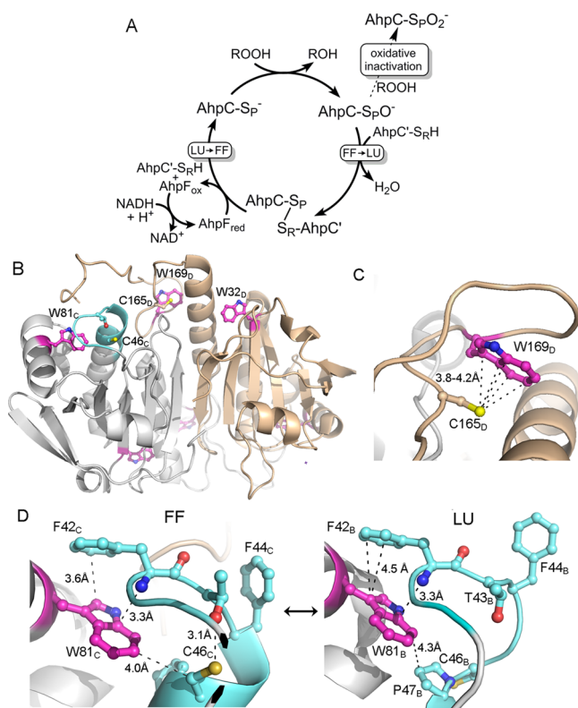
Figure 1. Catalytic cycle of 2-Cys peroxiredoxins and the location of the three Trp residues in Salmonella typhimurium AhpC. (A) The catalytic cycle (solid arrows) is shown along with the peroxide-mediated inactivation pathway (dashed arrow). The conformation change necessary for Prx catalysis is shown as a transition from fully folded (FF) to locally unfolded (LU) enzyme after sulfenyl formation at the peroxidatic Cys (shown as -S_pO^- ), and the opposite transition that occurs upon reduction of the disulfide bond between S_p and S_r (the sulfur group of the resolving Cys) to regenerate the active enzyme. Oxidative inactivation by peroxide can also occur at the peroxidatic Cys (dashed arrow) to generate the cysteine sulfinate (shown as -S_pO_2^- ). (B) A single dimer [taken from a 1.8 Å resolution decameric crystal structure of reduced, wild-type AhpC (Protein Data Bank entry 4MA9)] is depicted with chain D colored tan and the partner subunit (chain C) colored gray, highlighting the location of Trp residues (magenta), Cys residues, and the regions that undergo structural changes (cyan) during catalysis (sulfur atoms colored yellow, nitrogen atoms blue, and oxygen atoms red). (C) Close-up of the region around C165 in the FF conformation. In the LU conformation, W169 is presumed to be disordered as no electron density is observed for it. (D) Close-ups of the region around W81 in the FF and LU conformations. Selected residues and atomic distances (dashed lines) in panels C and D are shown with the same color scheme as in panel B. Subscript letters after the residue numbers indicate the subunit of that residue (described in ref 30). Shown to the right in panel D is the LU conformation only of subunit B in Protein Data Bank entry 4MA9.
