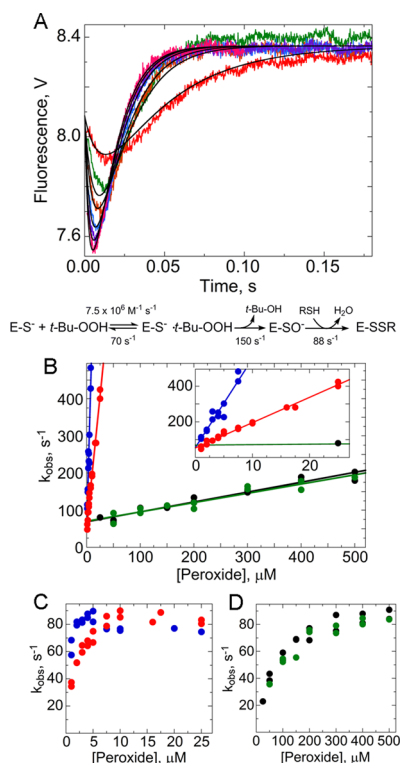
Figure 5. Rapid reaction kinetics of AhpC oxidation by various hydroperoxides. (A) Oxidation of wild-type AhpC by 50 (red), 150 (green), 200 (orange), 300 (blue), 400 (purple), and 500 \mu\text{M} tert -butyl hydroperoxide ( t -Bu-OOH) (magenta) monitored by Trp fluorescence. Methods used were identical to those described in the legend of Figure 2. Data were fit to a three-step model as in Figure 4, shown below the plot. In panels B–D, blue indicates data for \text{H}_2\text{O}_2 , red those for ethyl hydroperoxide, green those for t -Bu-OOH, and black those for cumene hydroperoxide. Results from two independent experiments are shown for each hydroperoxide. Panel B shows the rate of the fast, initial decrease for the four hydroperoxides, zooming in on values at low concentrations in the inset. Panels C and D show that all the substrates approach the same maximal rate for the exponential increase in fluorescence, with the slower substrates requiring higher concentrations.
